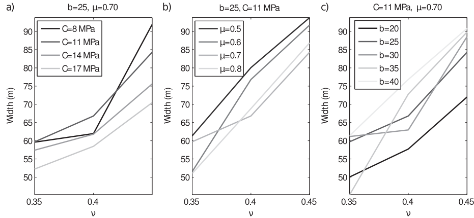
Figure 13. Effects of mechanical parameters on the width of the damaged zone ( W ). The coupled effect of the Poisson's ratio and (a) the cohesion, (b) the friction, (c) the b parameter.
